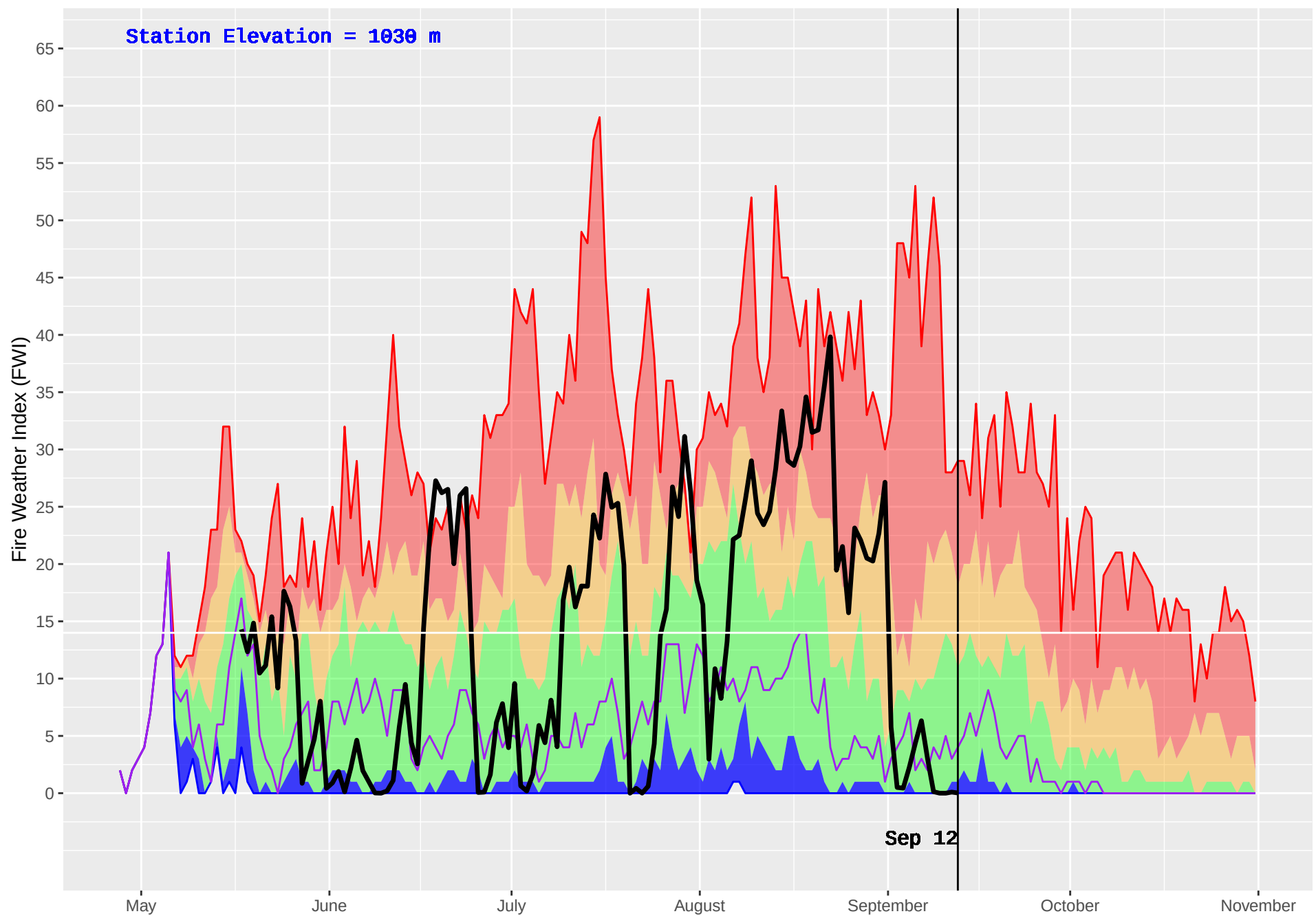
WITCH (154) : Historical (1993–2016) and Current (2018) Daily Fire Weather Index (FWI)
