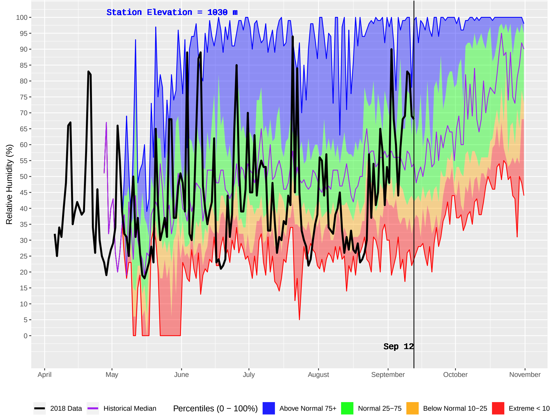
WITCH (154) : Historical (1993–2016) and Current (2018) Daily Relative Humidity
