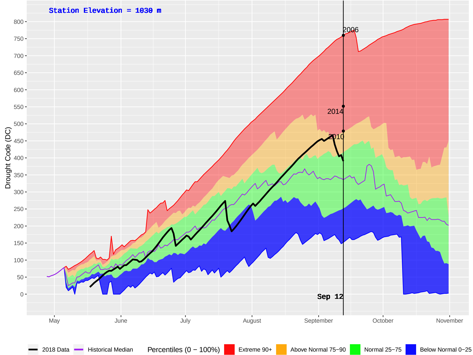
WITCH (154) : Historical (1993–2016) and Current (2018) Daily Drought Code (DC)
