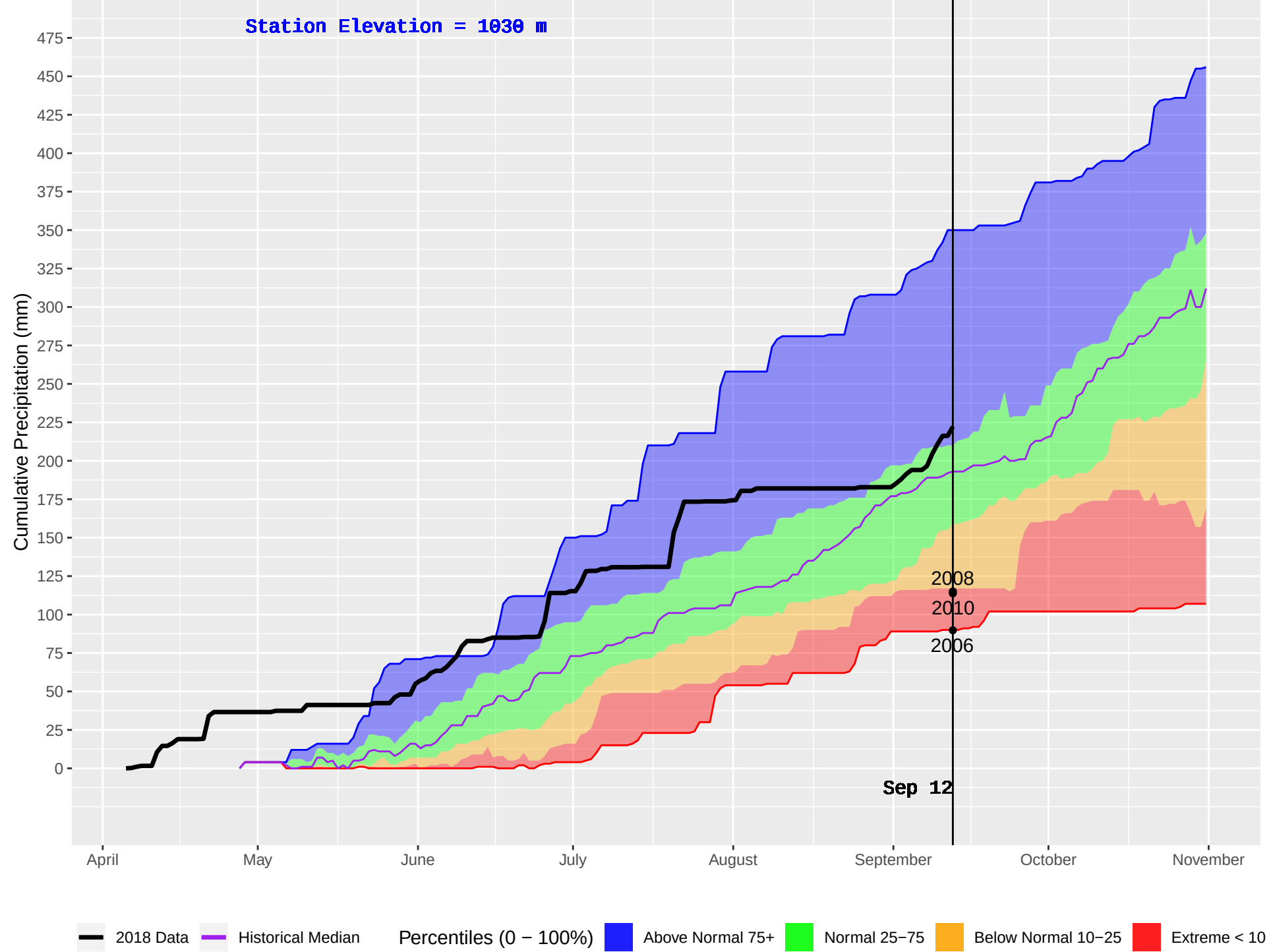
WITCH (154) : Historical (1993–2016) and Current (2018) Daily Cumulative Precipitation
