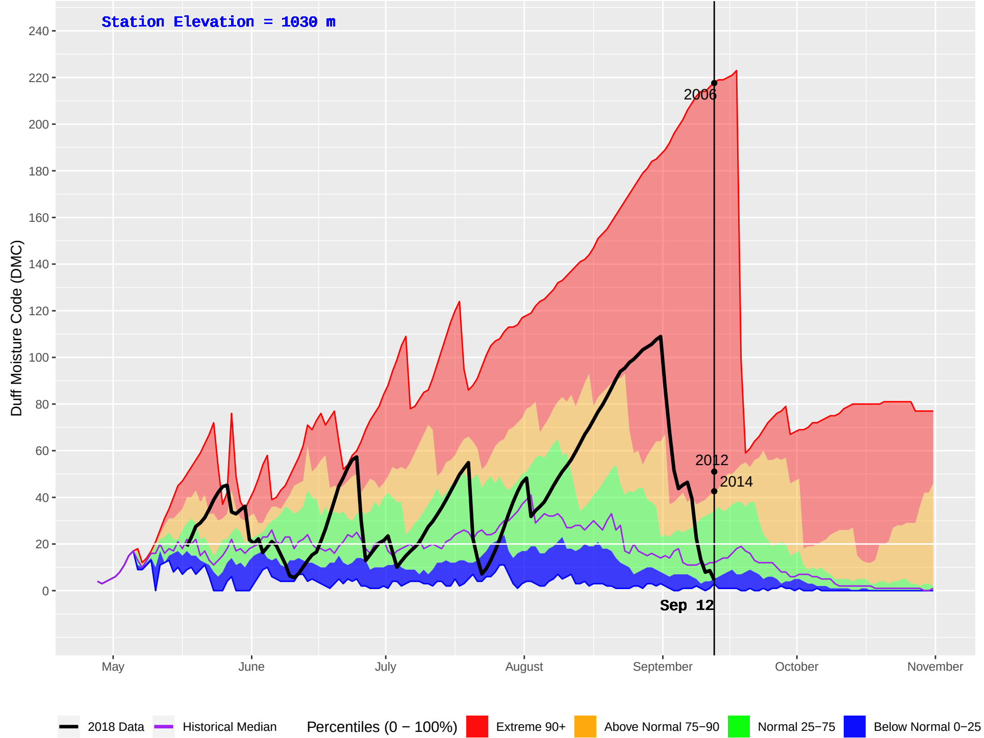
WITCH (154) : Historical (1993–2016) and Current (2018) Daily Duff Moisture Code (DMC)
