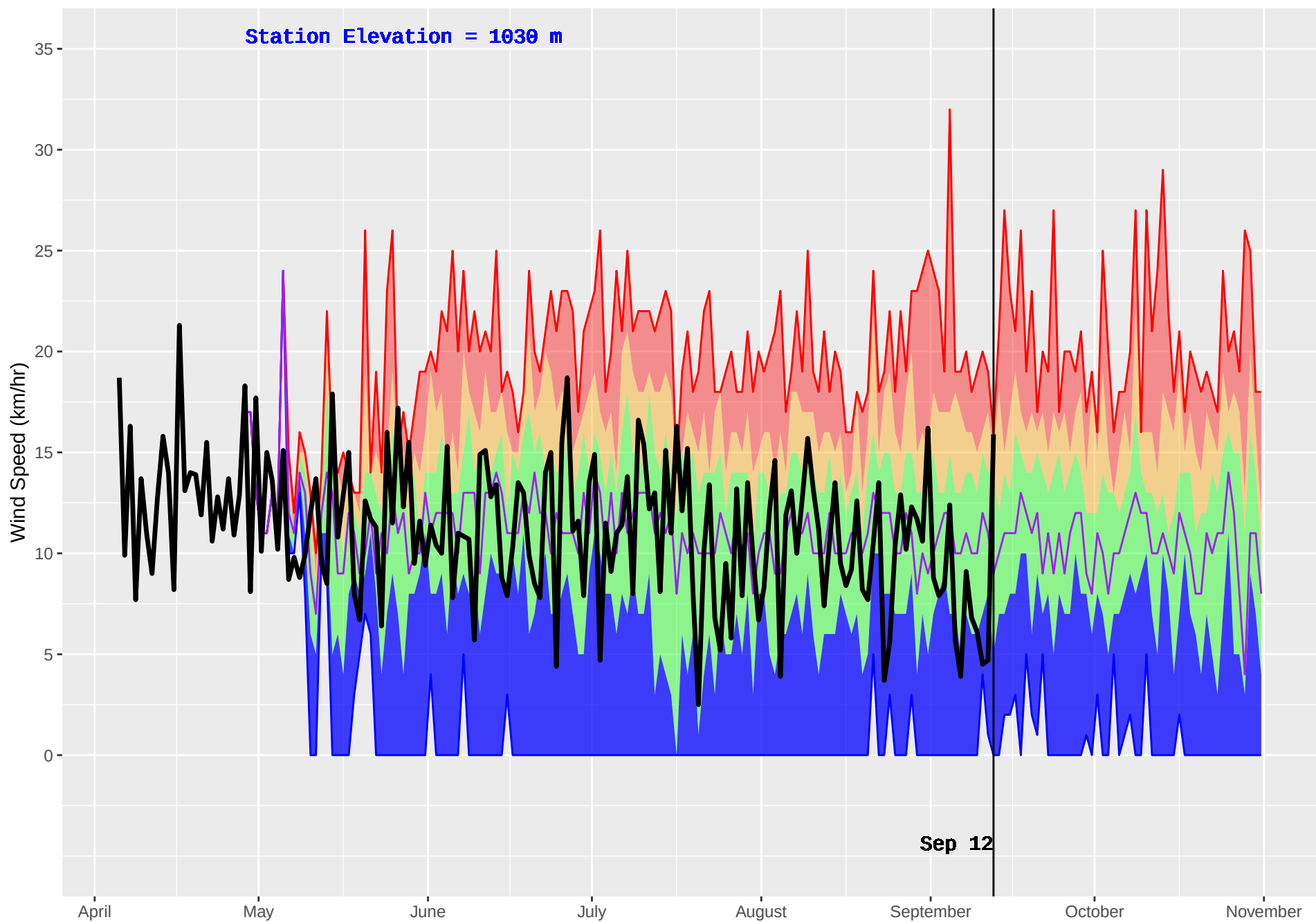
WITCH (154) : Historical (1993–2016) and Current (2018) Daily Wind Speed
