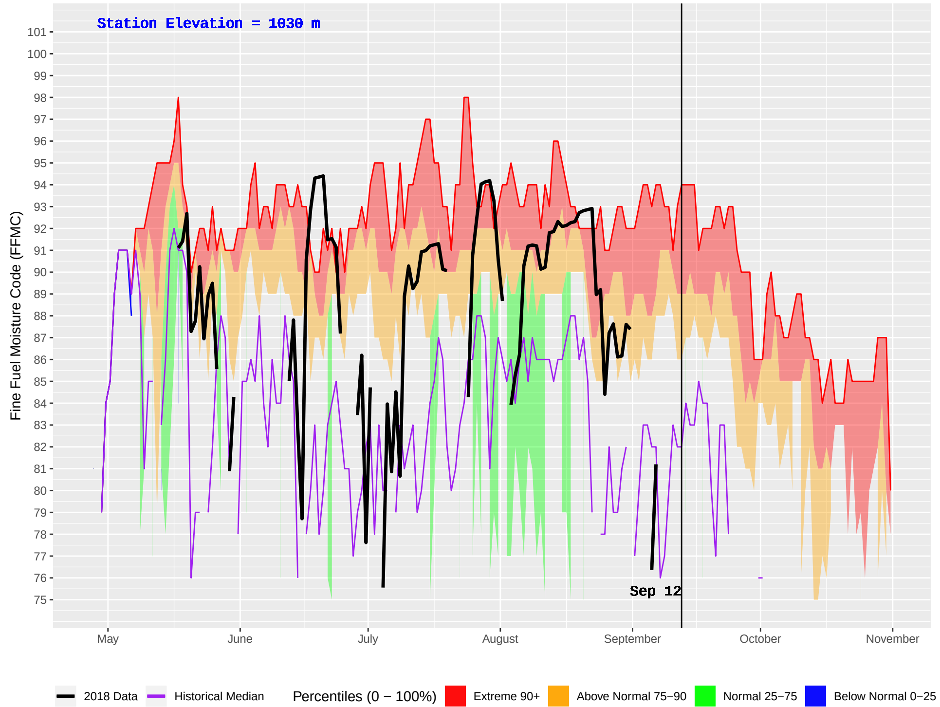
WITCH (154) : Historical (1993–2016) and Current (2018) Daily Fine Fuel Moisture Code (FFMC)
