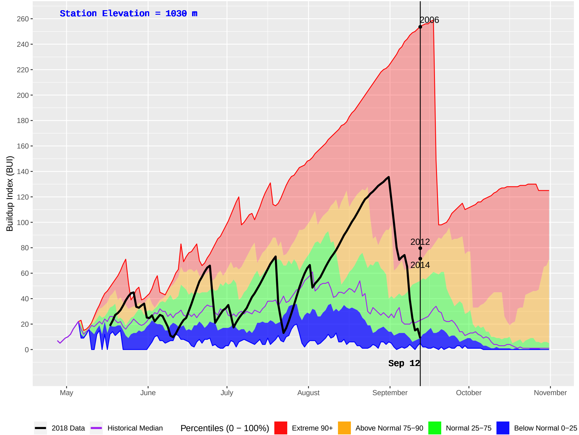
WITCH (154) : Historical (1993–2016) and Current (2018) Daily Buildup Index (BUI)
