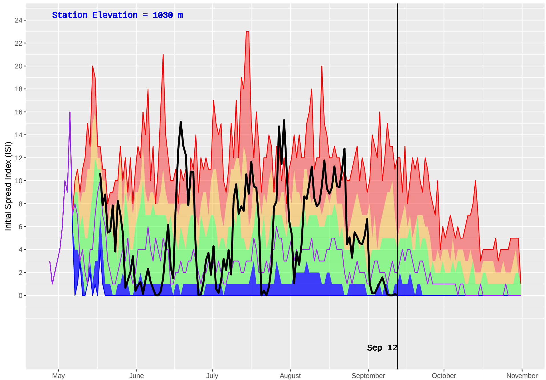
WITCH (154) : Historical (1993–2016) and Current (2018) Daily Initial Spread Index (ISI)
