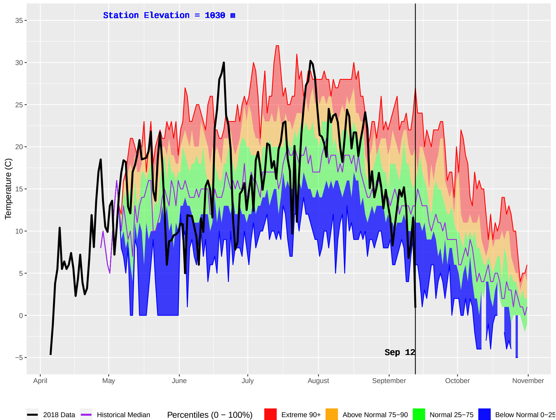
WITCH (154) : Historical (1993–2016) and Current (2018) Daily Temperature
